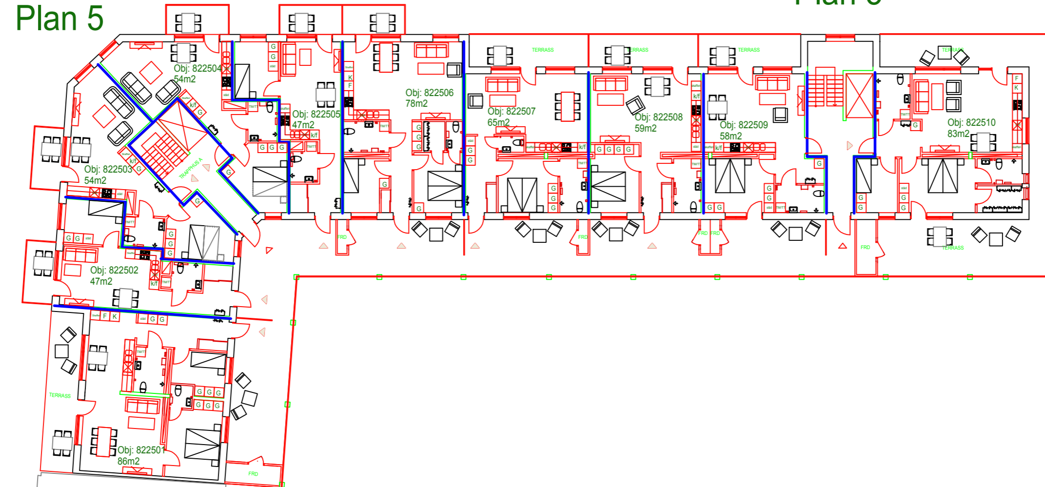
Plan 5
